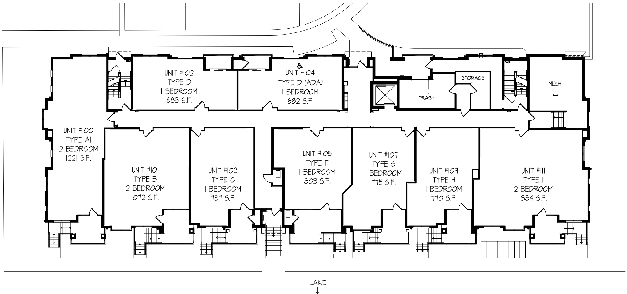
FIRST FLOOR PLAN WINGRA SHORES APARTMENTS 2628 ARBOR DRIVE
